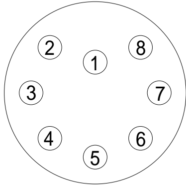
OM8FSX Underwater connector view on sockets
